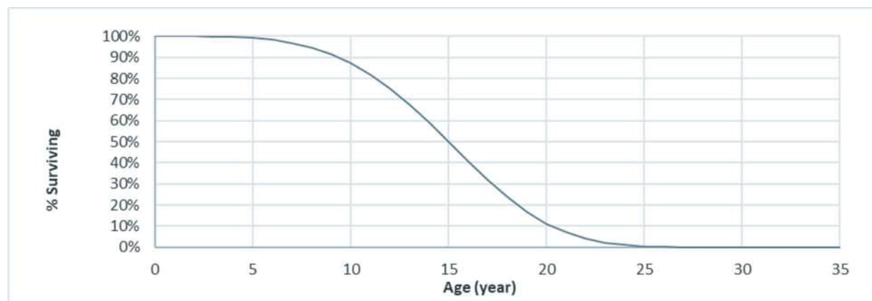
Figure 2-1 Survival Function for Premium Efficiency Motors 296
