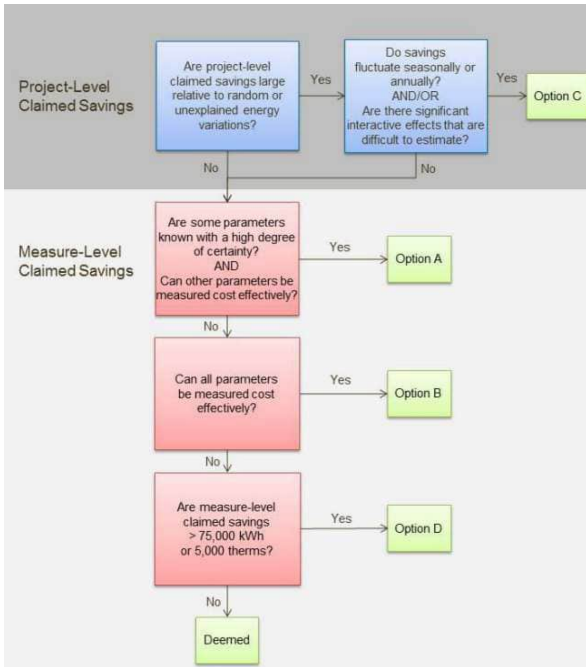
Figure 2-7 RCx Decision Flow Chart 43
