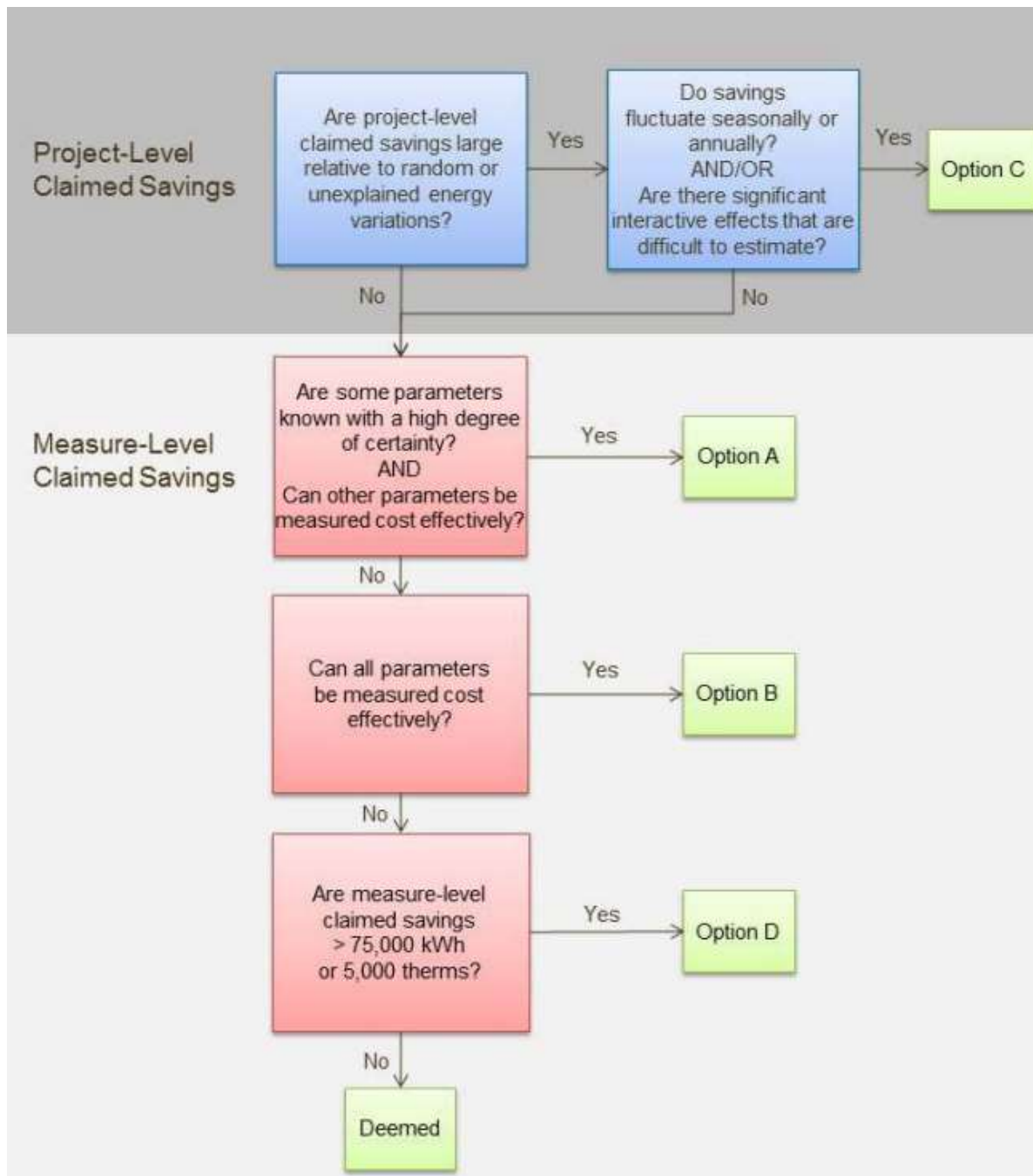
Figure 2-7 RCx Decision Flow Chart 40
