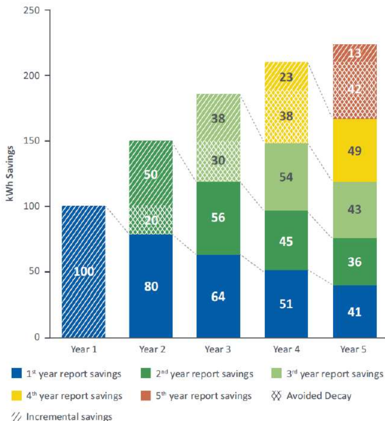
Figure 2-14 Illustration of Savings Persistence 108
