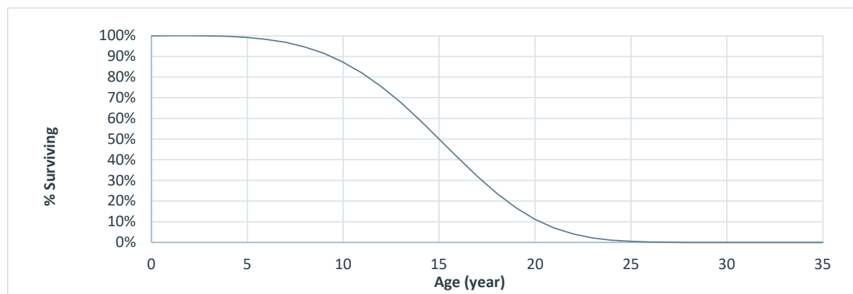
Figure 2-1 Survival Function for Premium Efficiency Motors 255
