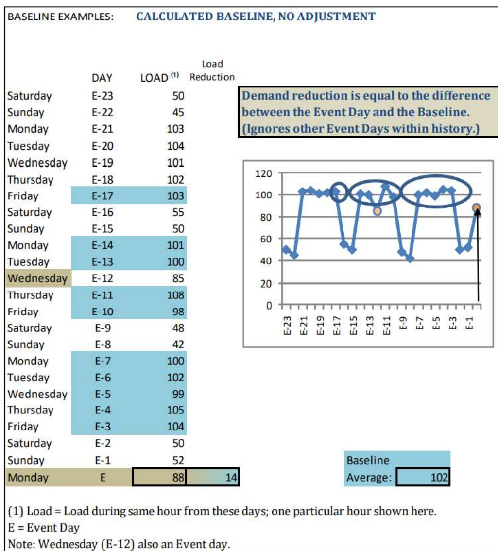
Figure 1-1 Calculated Baseline, No Adjustment 27
