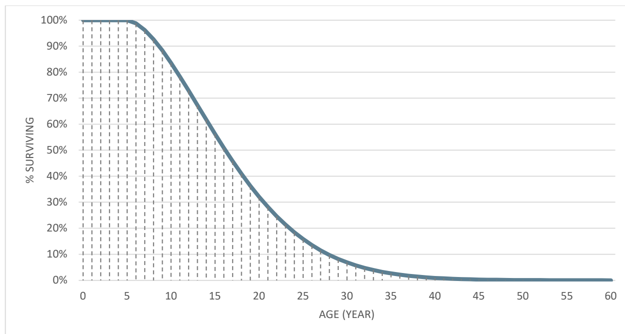
Figure 1-2 Survival Function for ENERGY STAR Refrigerators 52
