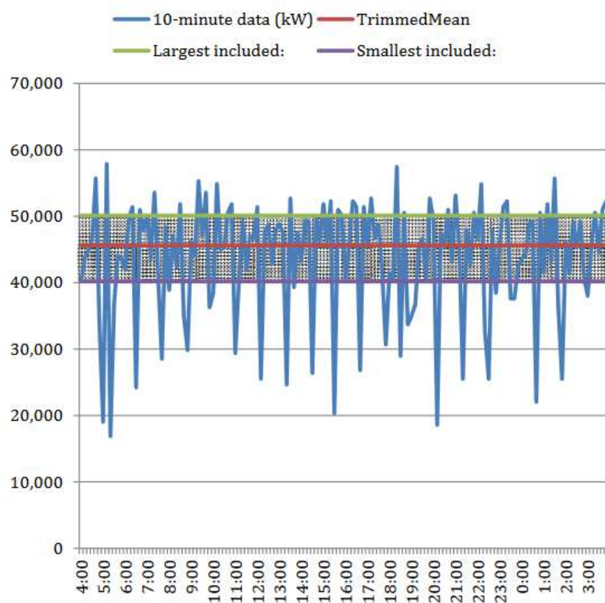
Figure 2-24 Consumption Trimming
