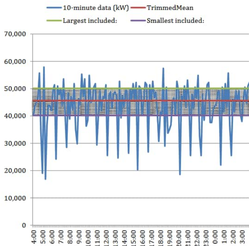
Figure 2-24 Consumption Trimming
