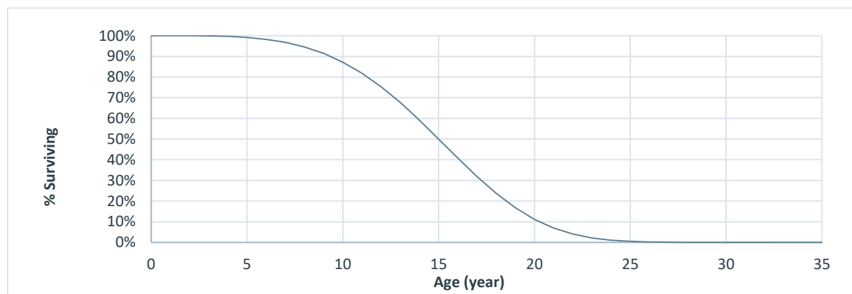
Figure 2-1 Survival Function for Premium Efficiency Motors 195
