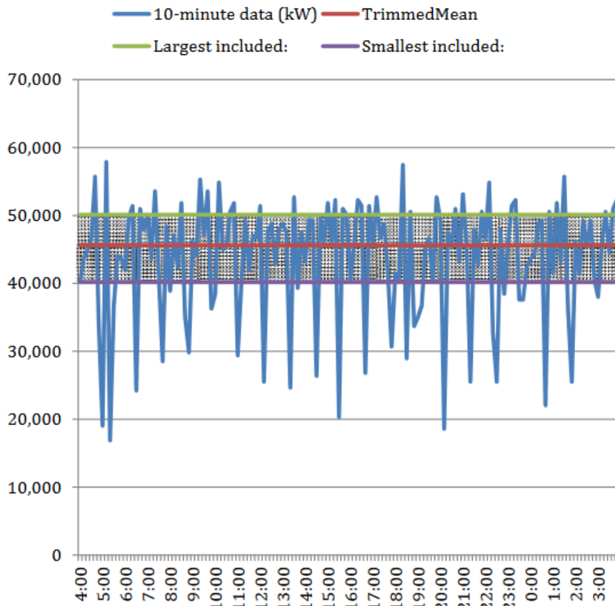
Figure 2-24 Consumption Trimming
